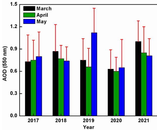
Fig. 7. Pre-monsoonal variation in AOD in 550 nm for the period of June 2017 to May 2021 over Guwahati.
