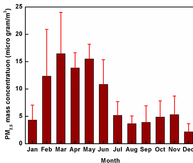
Fig. 5. Monthly variation in PM 2.5 mass concentration for the period of June 2017 to May 2021 over Guwahati.
