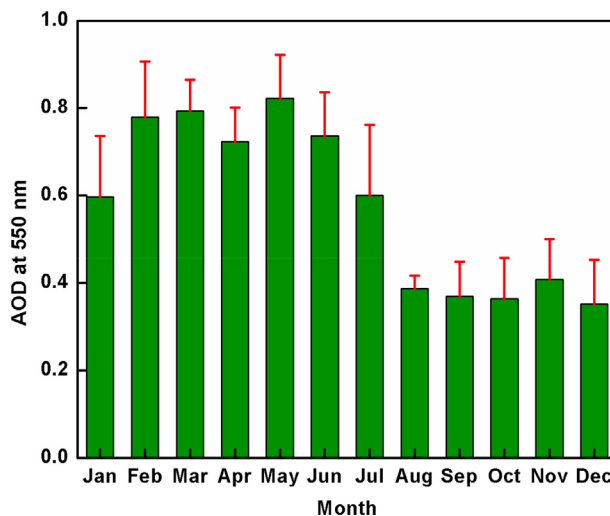
Fig. 3. Monthly variation in MODIS AOD at 550 nm for the period of June 2017 to May 2021 over Guwahati.
